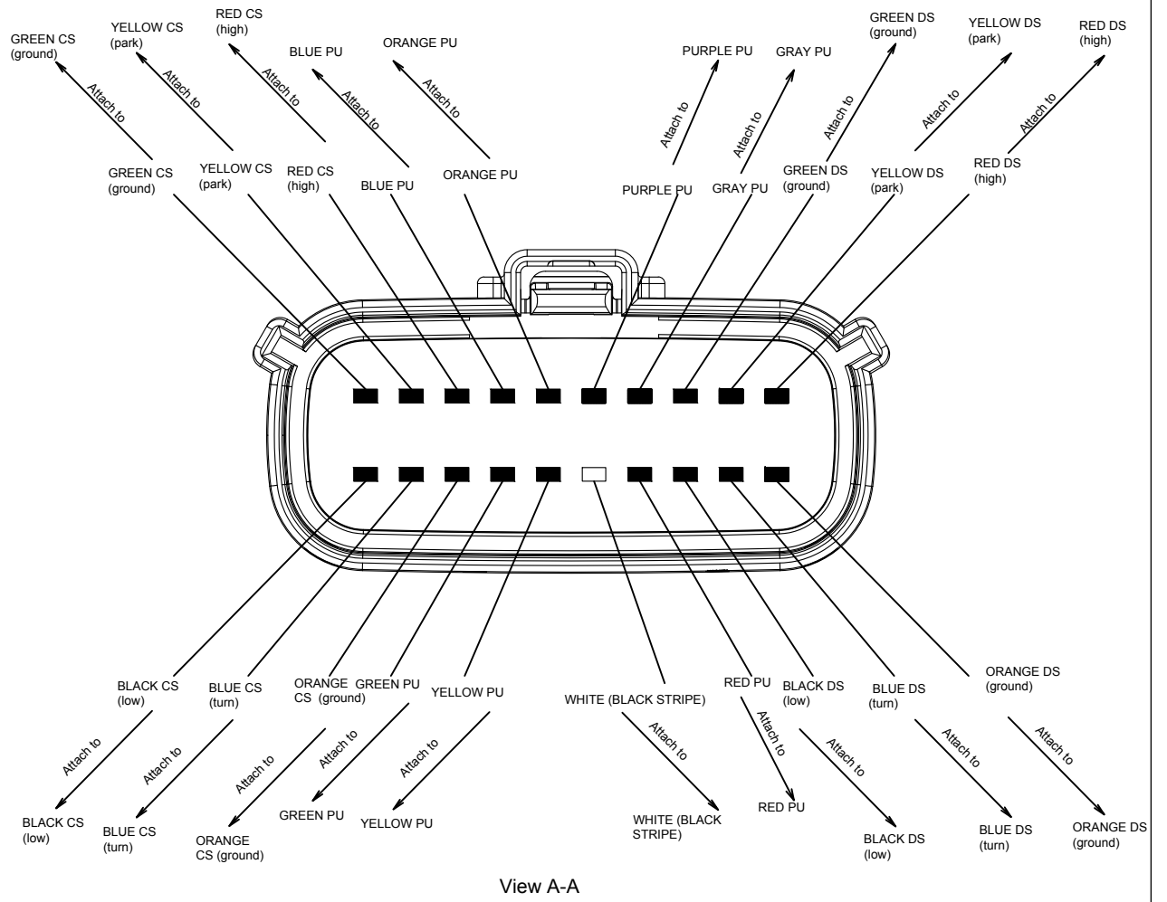
One piece harness Connector Truck Side
